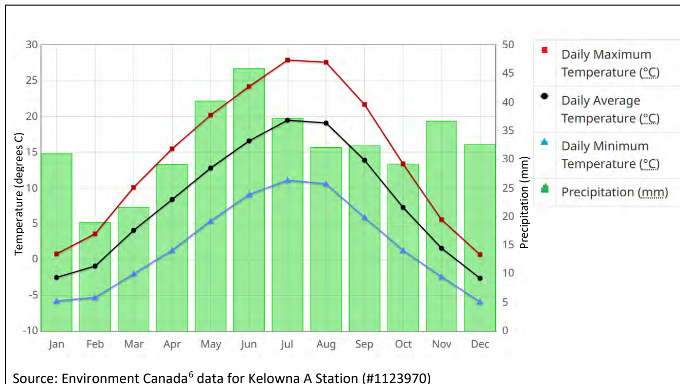
Figure 4-2: Temperature and Precipitation Climate Normals (1981-2010) for Kelowna A, BC
