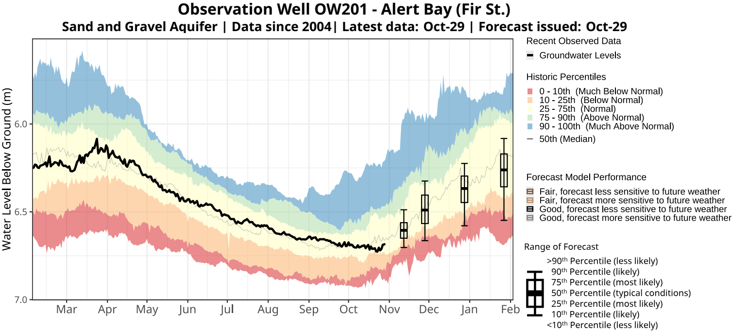
OW201 - Likelihood (%) of Groundwater Level Conditions
