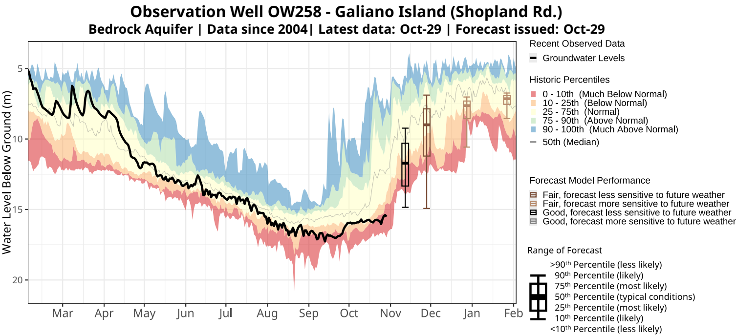
OW258 - Likelihood (%) of Groundwater Level Conditions
