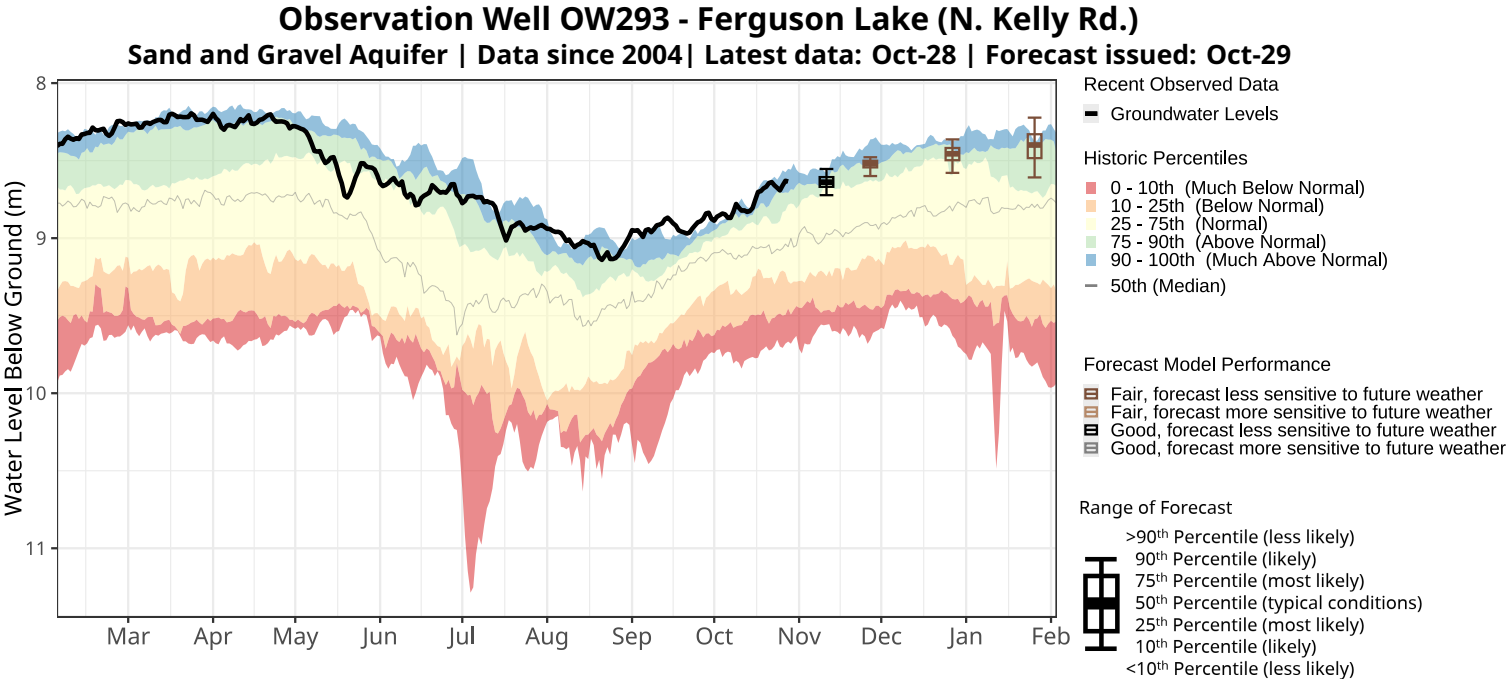
OW293 - Likelihood (%) of Groundwater Level Conditions
