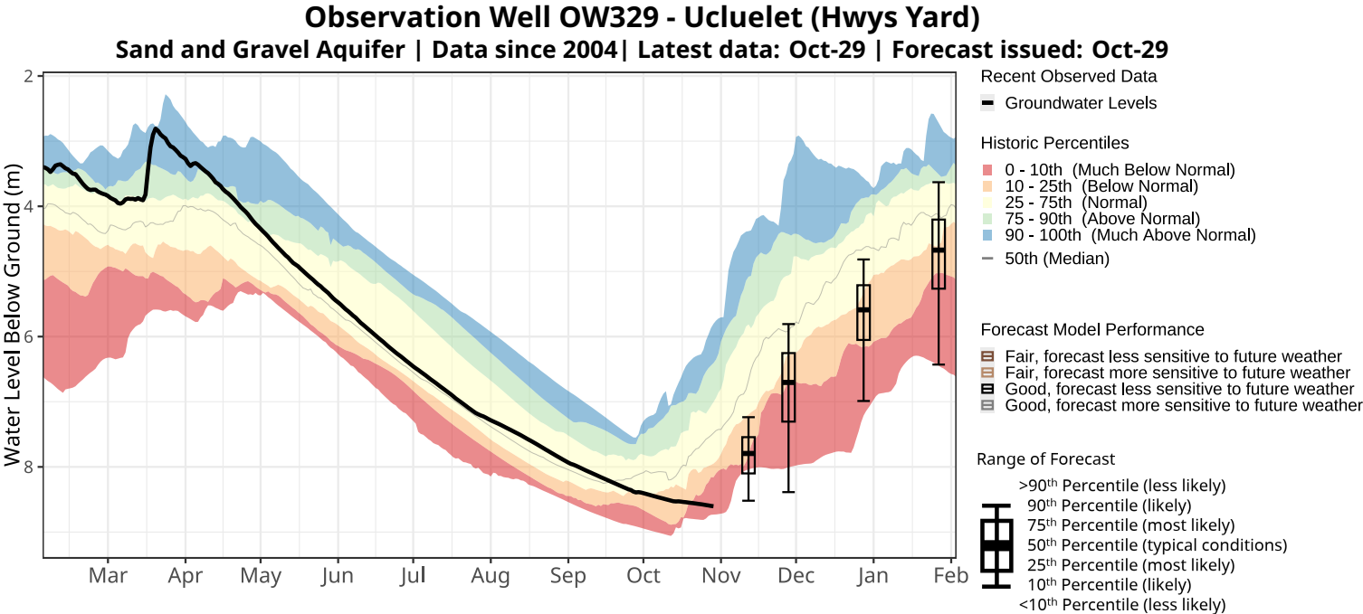
OW329 - Likelihood (%) of Groundwater Level Conditions
