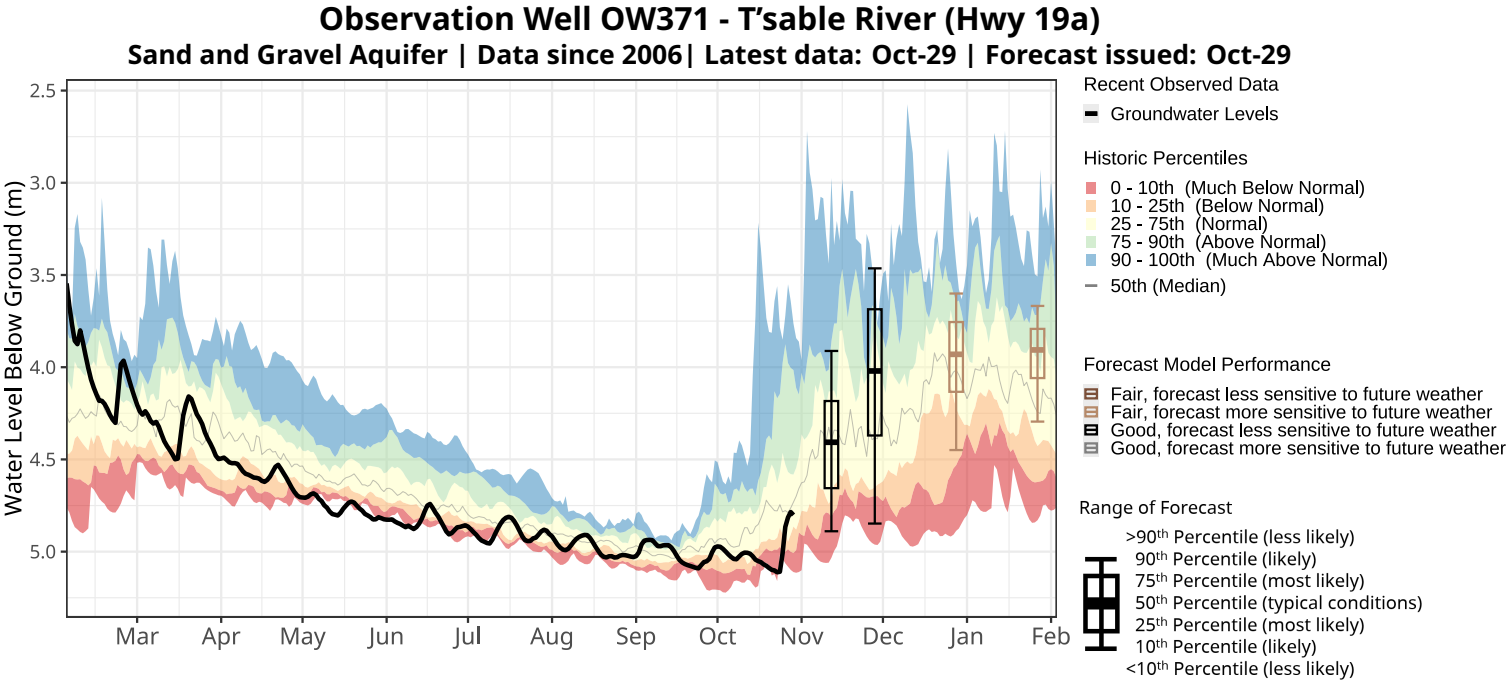
OW371 - Likelihood (%) of Groundwater Level Conditions
