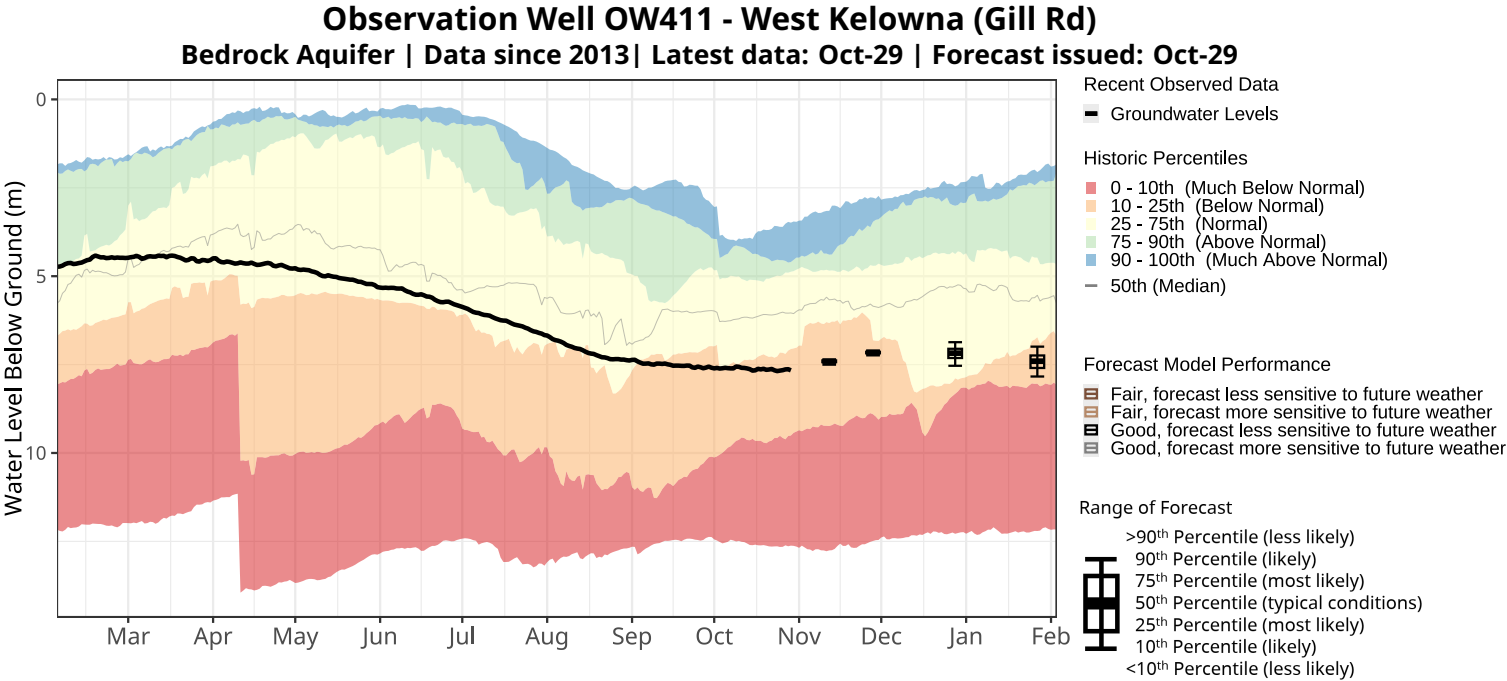
OW411 - Likelihood (%) of Groundwater Level Conditions
