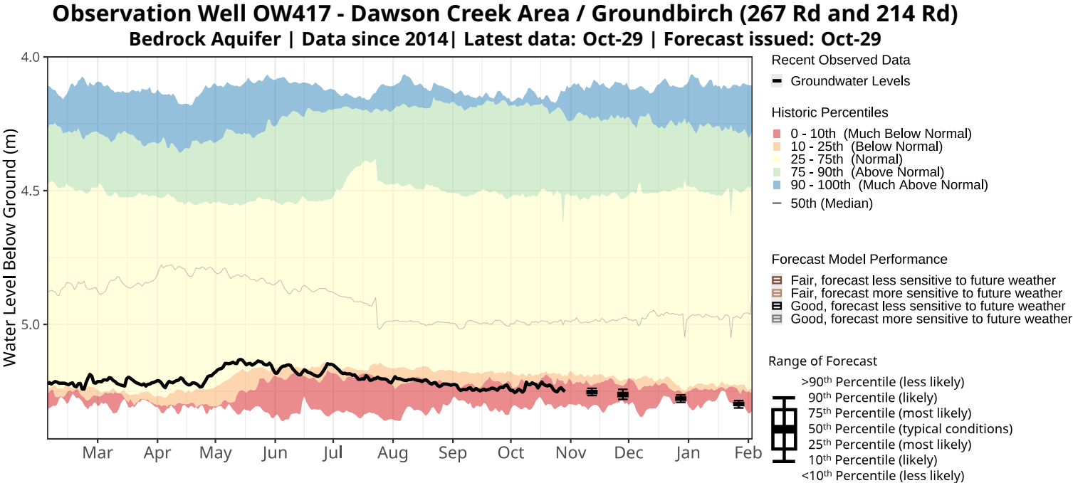
OW417 - Likelihood (%) of Groundwater Level Conditions
