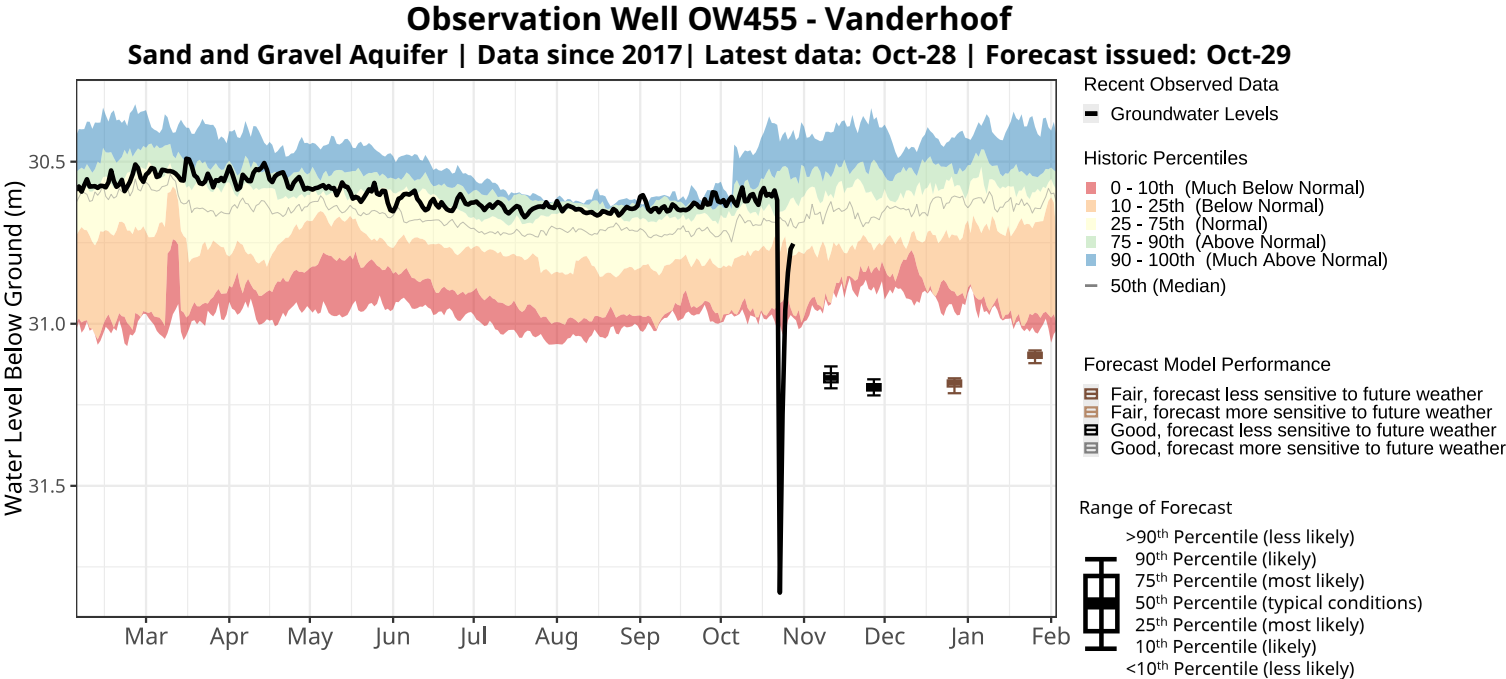
OW455 - Likelihood (%) of Groundwater Level Conditions
