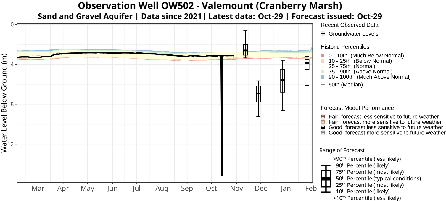
OW502 - Likelihood (%) of Groundwater Level Conditions
